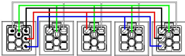
Phase Tap 3L,N,G (347/600V shown)
