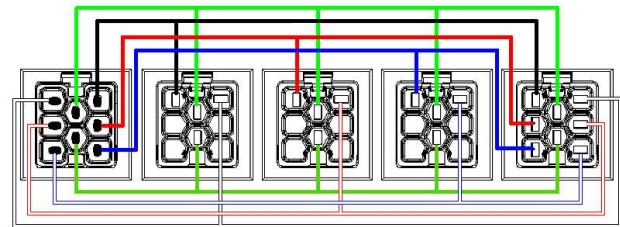
Phase Tap 3L,3N,2G (347/600V shown)
