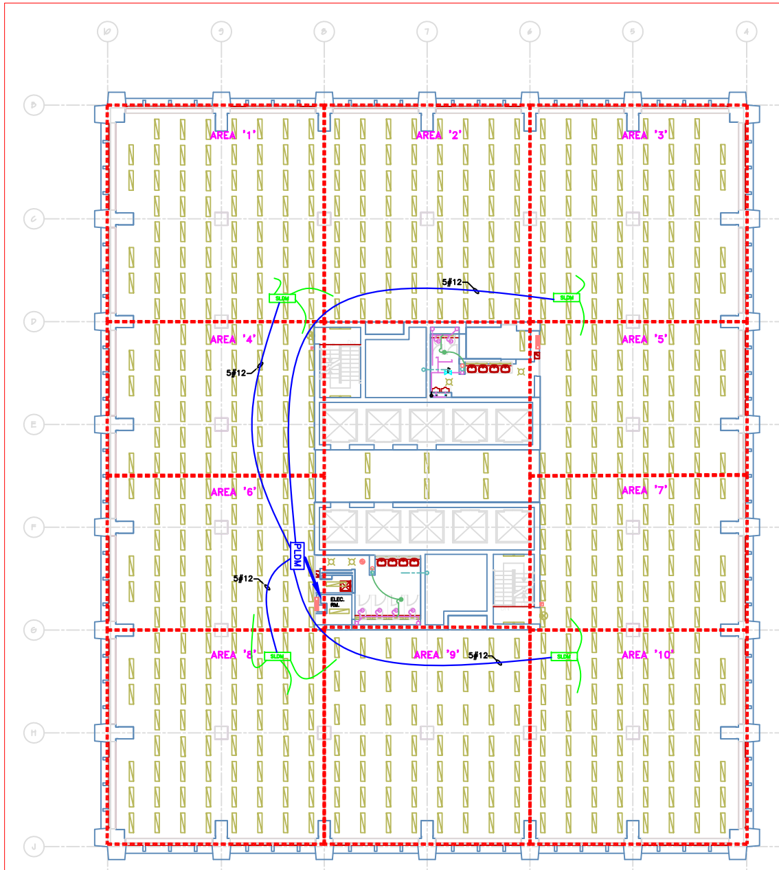
347V LIGHTING LAYOUT SCALE 1 : 100
