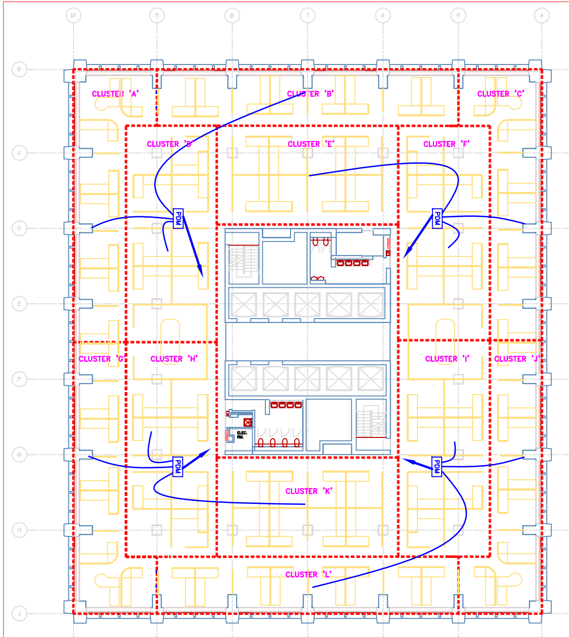
1 UNIVERSAL POWER DISTRIBUTION LAYOUT SCALE 1 : 100
